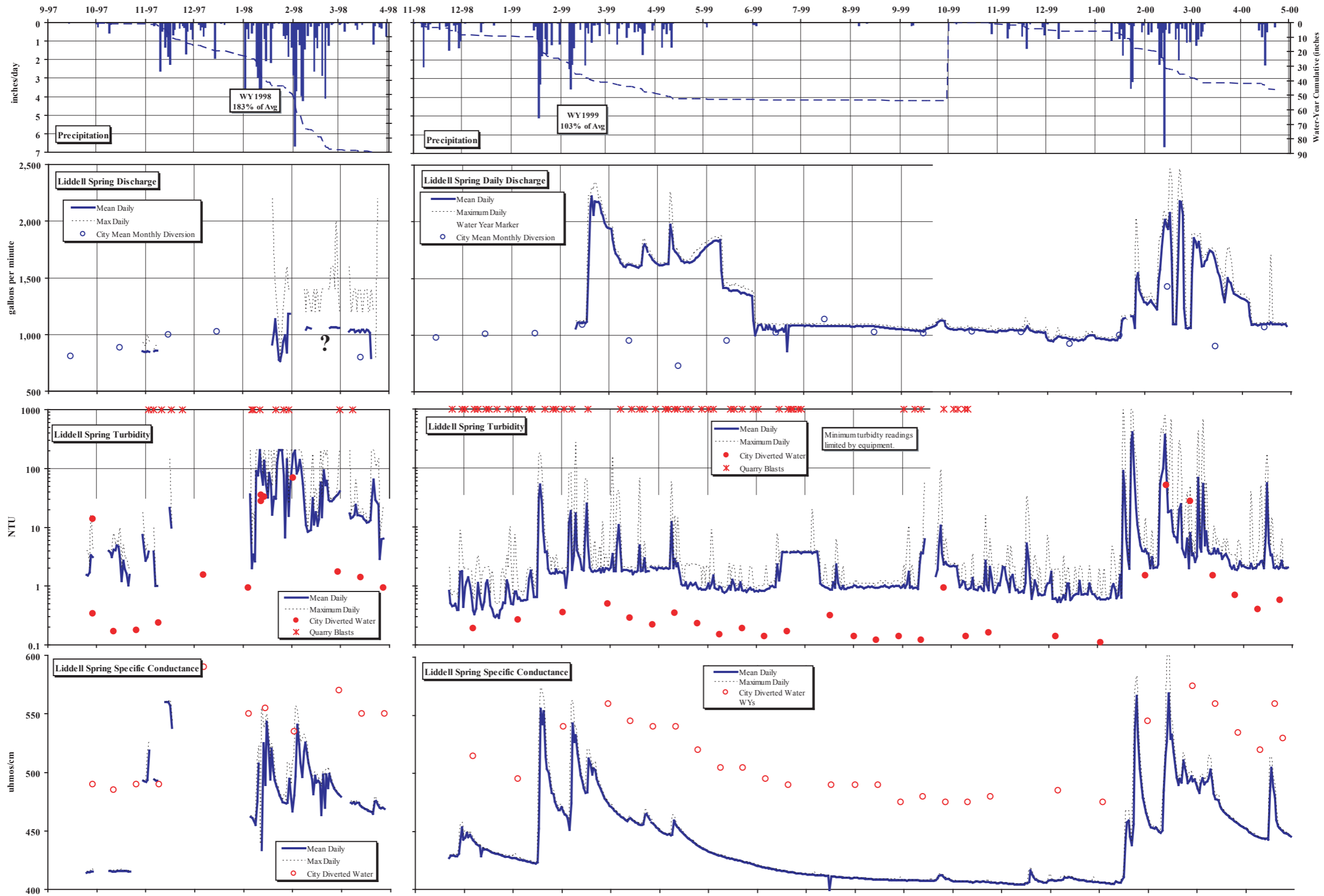
Liddel Spring Data Logger Record for Discharge, Turbidity, Specific Conductance, and Precipitation, September 1997 - May 2000
